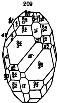
Humite.
